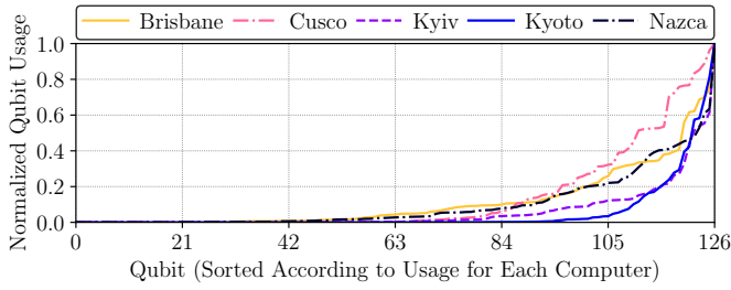
Fig. 3: Our analysis indicates that across all quantum computers, a small set of qubits gets used more frequently.
