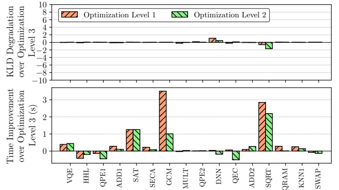
Fig. 6: Optimization levels 1 and 2 achieve similar KLD values as optimization level 3, while achieving much lower transpilation time than optimization level 3.
